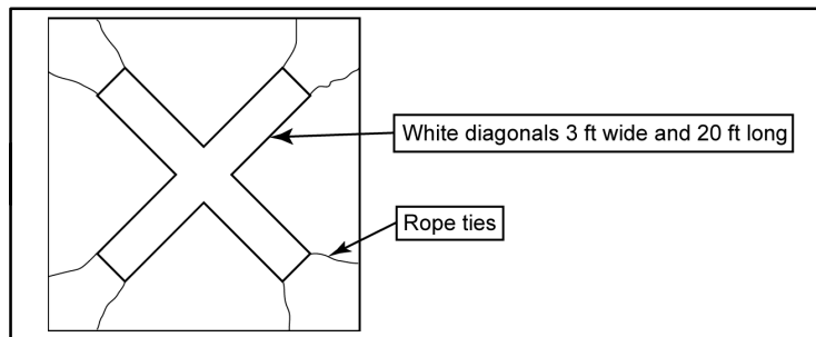
FIG 10–2–2 Closed Helideck Marking
