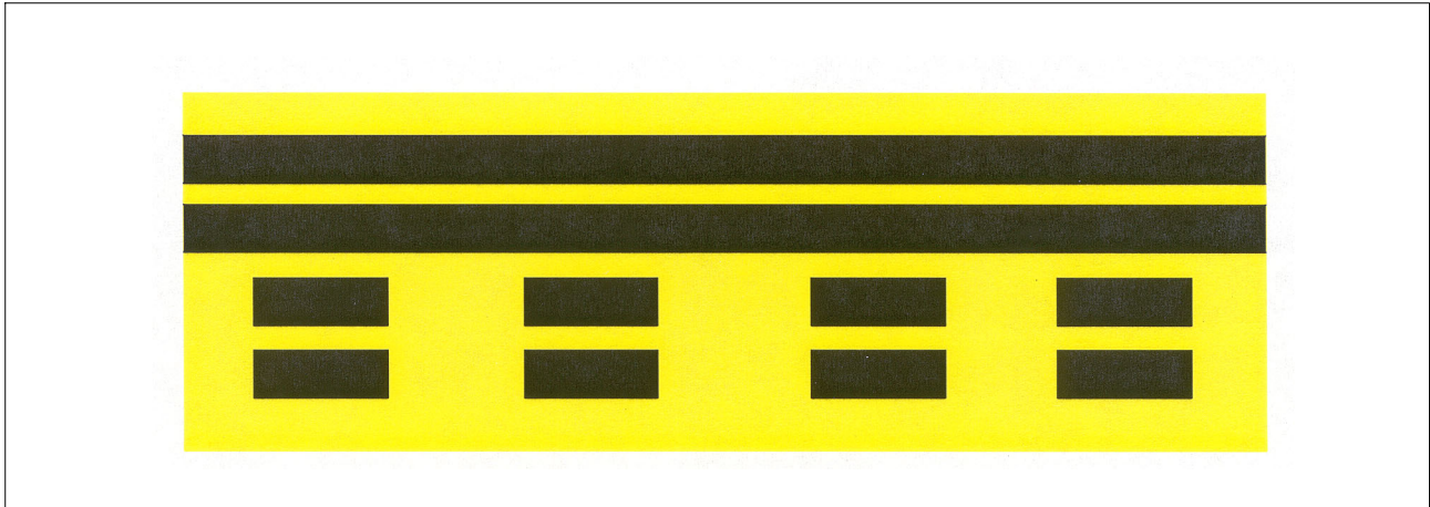
FIG 2-3-33 Runway Boundary Sign
