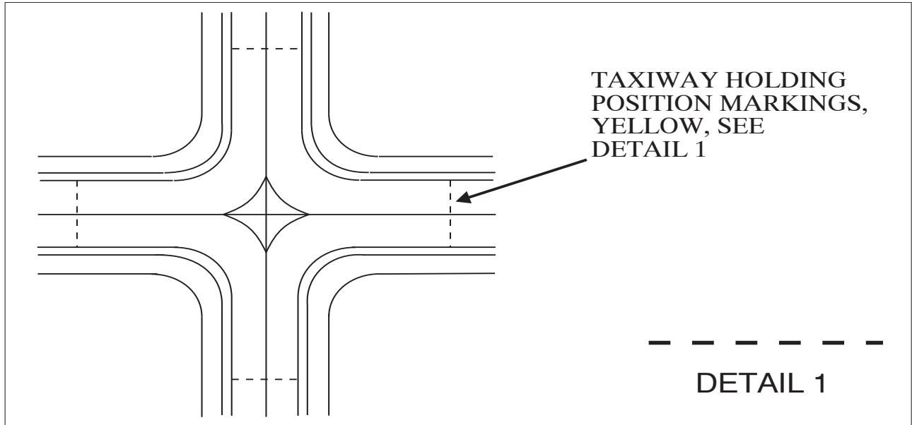
FIG 2-3-17 Holding Position Markings: Taxiway/Taxiway Intersections
