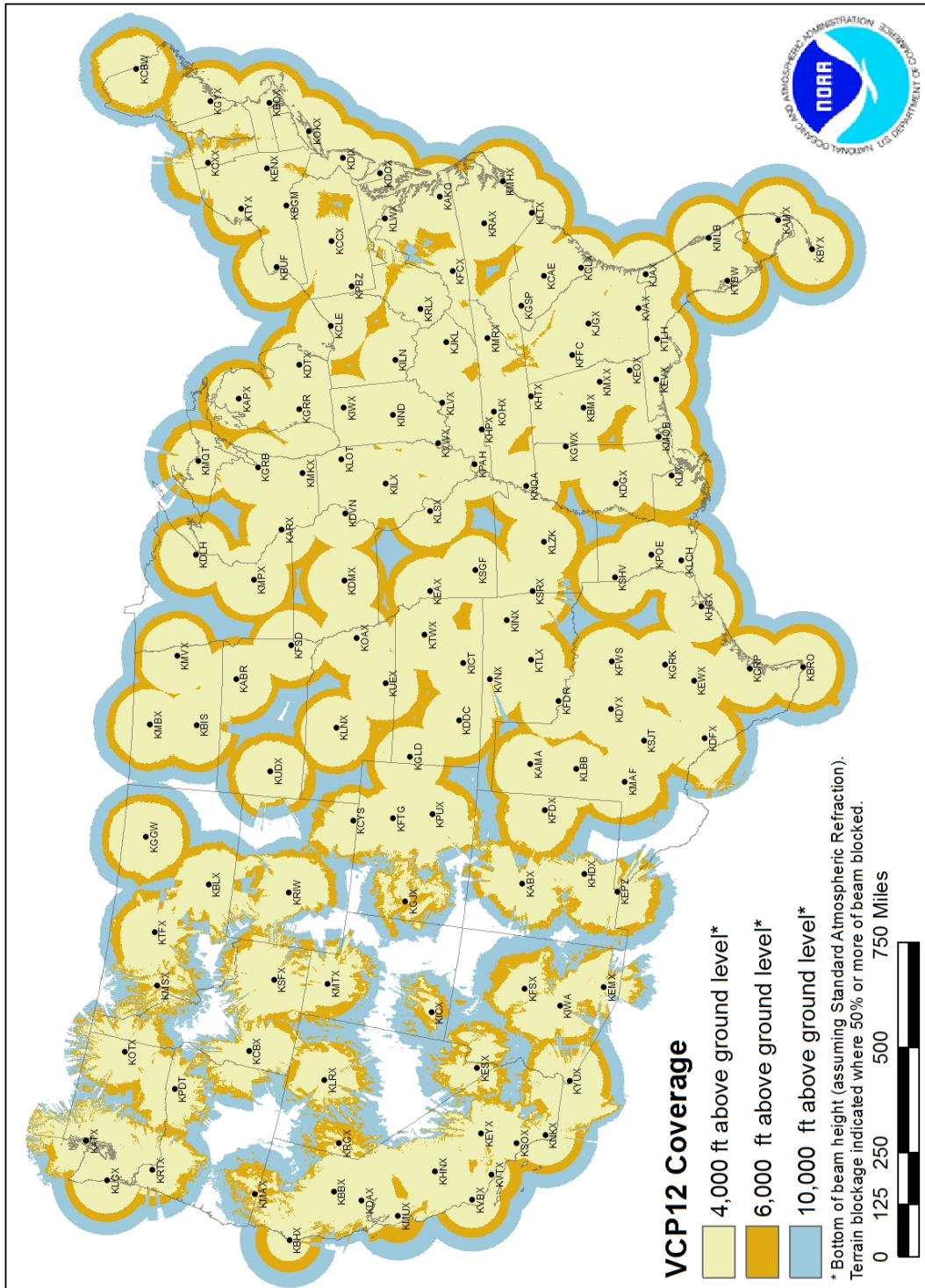
FIG 7-1-10 NEXRAD Coverage
