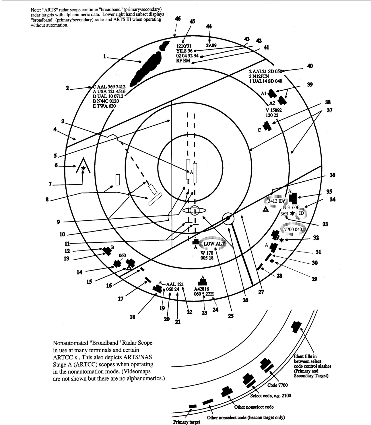
FIG 4-5-3 ARTS III Radar Scope With Alphanumeric Data
