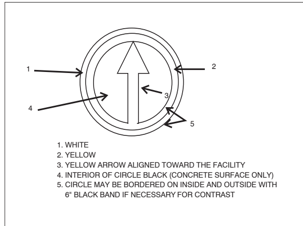
FIG 2-3-21 Nonmovement Area Boundary Markings
