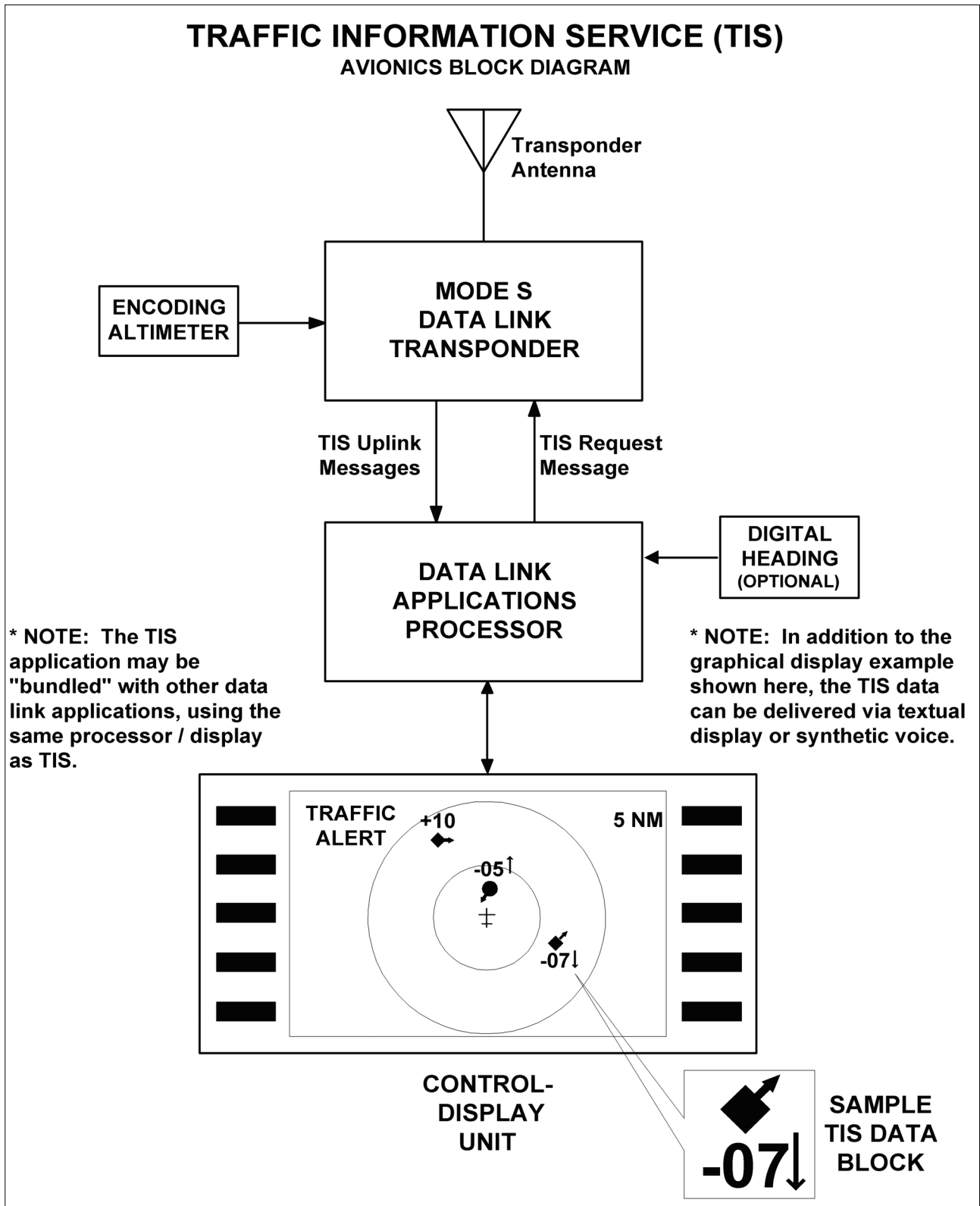
FIG 4-5-7 Traffic Information Service (TIS) Avionics Block Diagram
