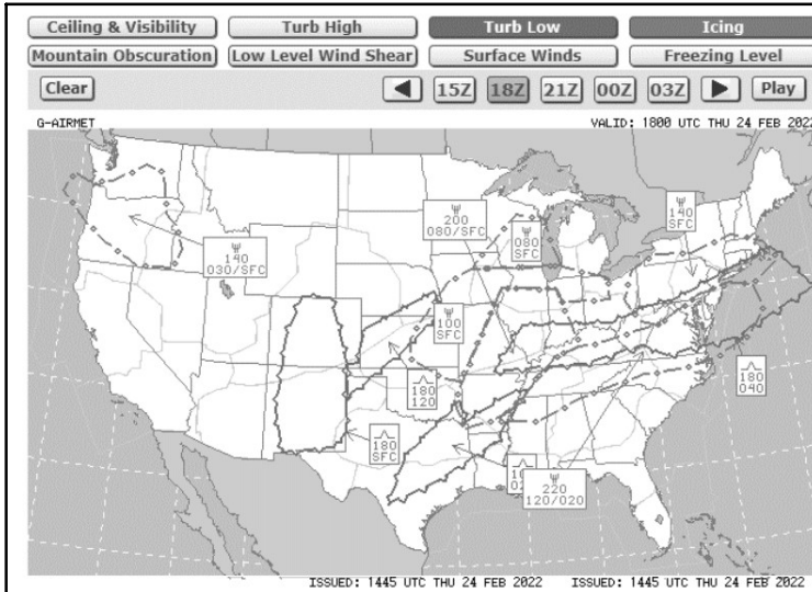
FIG 7-1-7 AIRMET over the Contiguous U.S.
