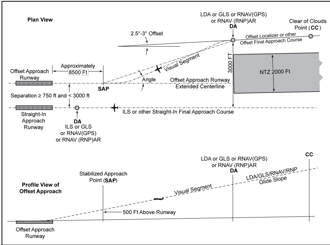
FIG 5-4-25 SOIA Approach Geometry
