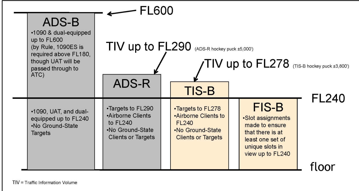
FIG 4-5-10 Terminal – ADS-B/ADS-R/TIS-B/FIS-B Service Ceilings/Floors
