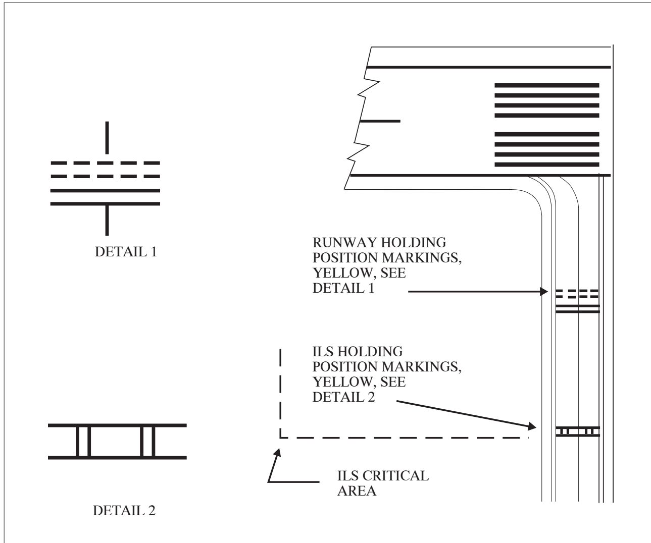
FIG 2-3-16 Holding Position Markings: ILS Critical Area
