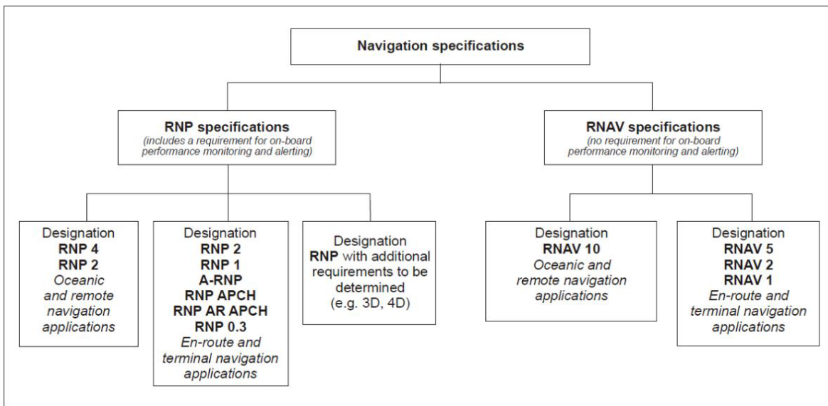
FIG 1-2-1 Navigation Specifications
